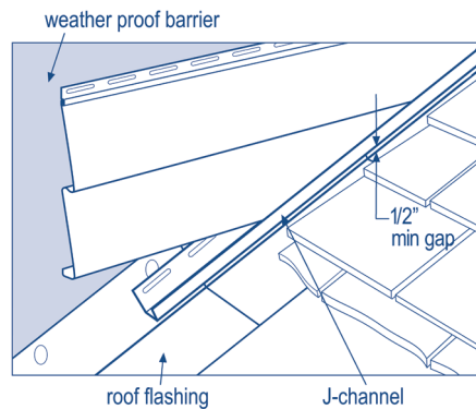
Installation over roof line
