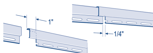
Splicing of the undersill trim
