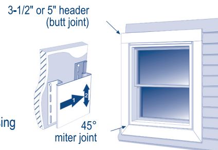
Window corner detail
