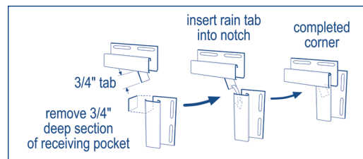
Corner detail A - Square corner
