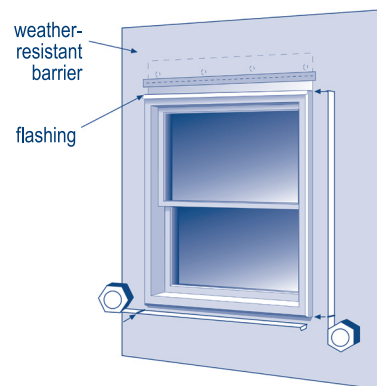
Window detail
