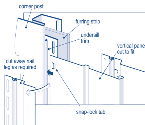
Alternate wall ending
