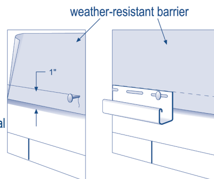
Starting the wall
