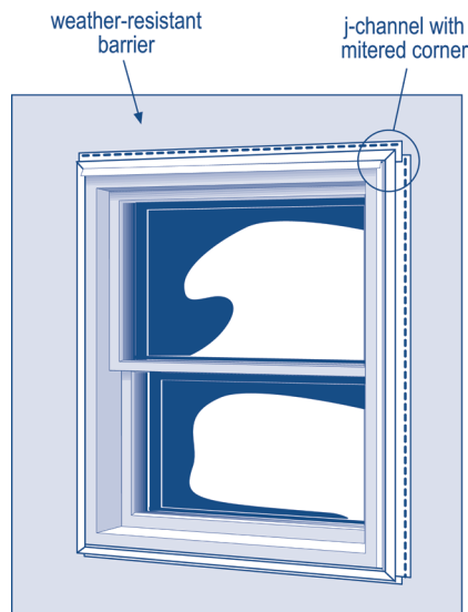
Window detail
