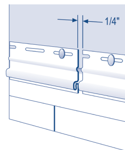
Starter trim installation
