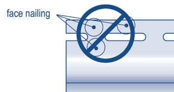
Position of fasteners
