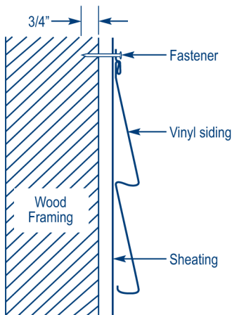
New construction
