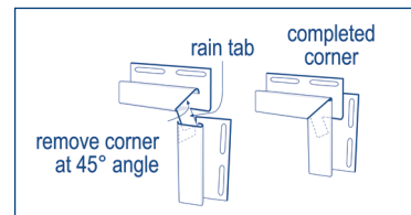
Corner detail B - Mitered corner
