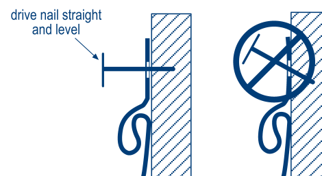
Fasteners detail
