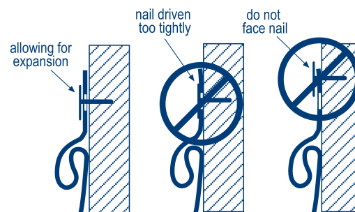
Nailing guidelines
