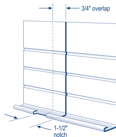
Fascia overlapping
