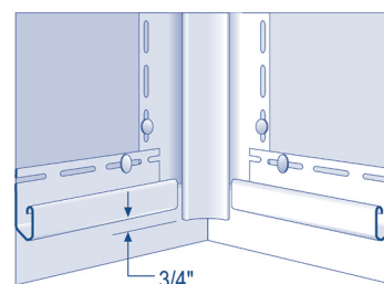
Inside corner detail
