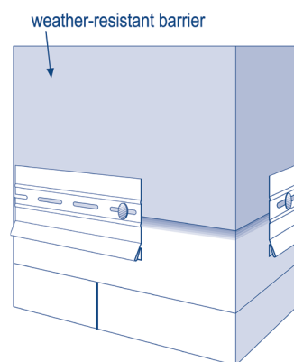
Starter trim at corners
