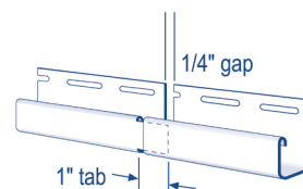
Splicing J-channels
