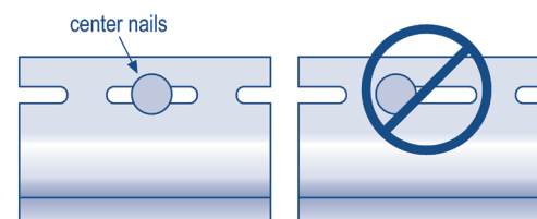
Nailing guidelines
