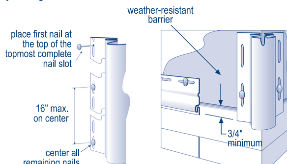
Quarter round corner starter installation
