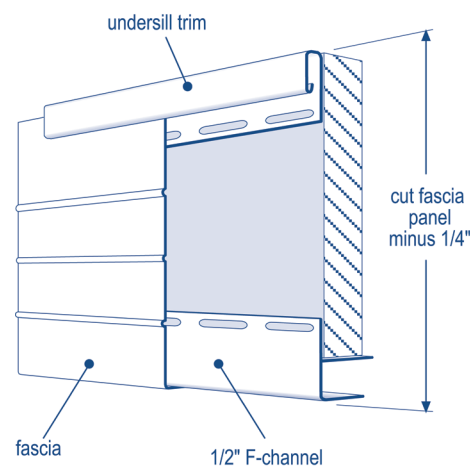
Fascia installation
