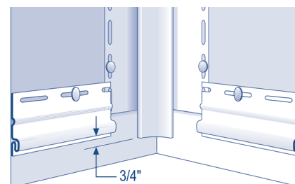
Starter trim and inside corner post
