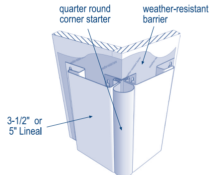
Assembled Lineal corner
