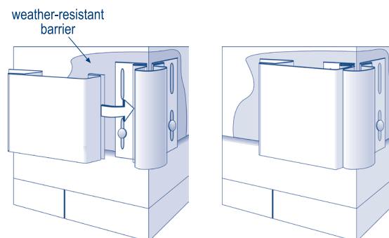
Side Lineal installation
