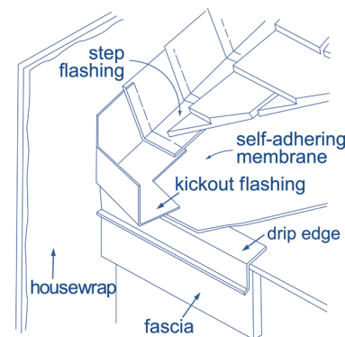
Side wall flashing
