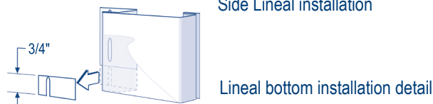
Side Lineal installation
