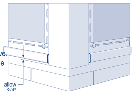
Outside corner detail
