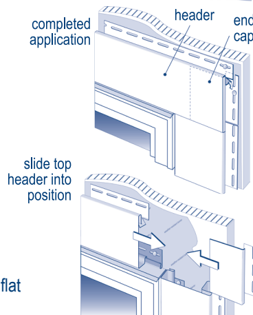
Assembly Lineal corner detail
